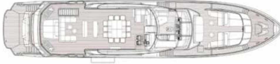
DECK PLAN
